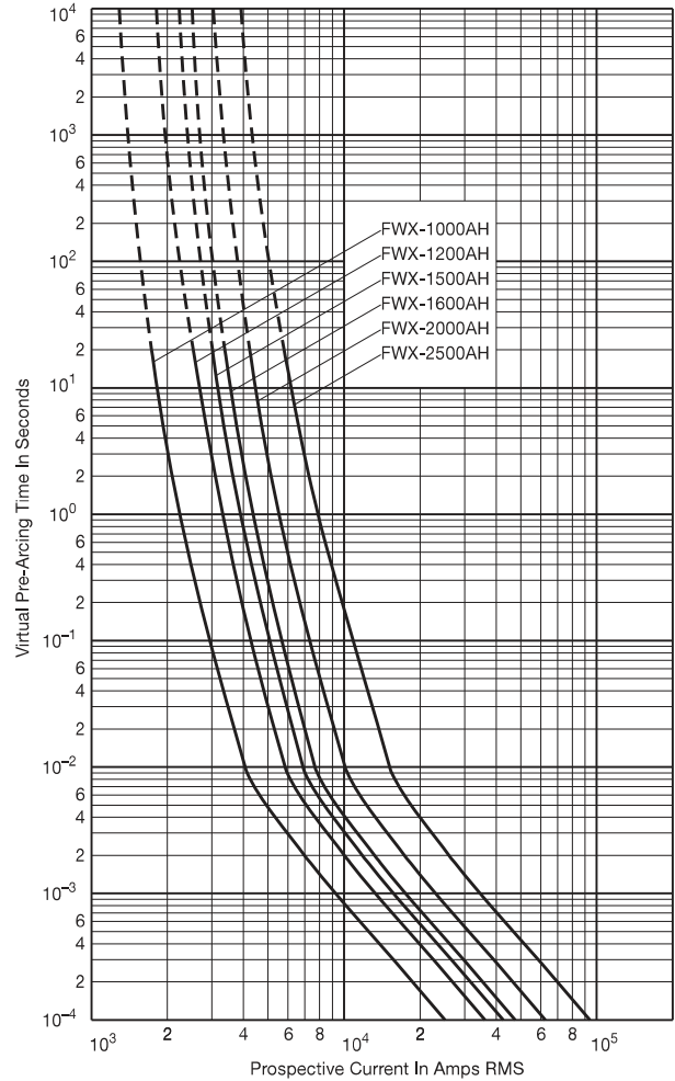
Time-Current Curve
