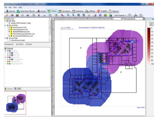
Figure 8: 802.11n heat map
