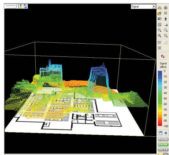
Figure 3: 3D view to visualize highest/lowest signal
